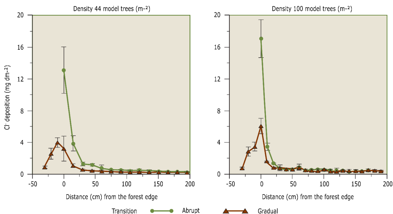
Figure 48-8: Dry deposition of Cl - (chloride) along a transect running from the forest edge to the stock in
